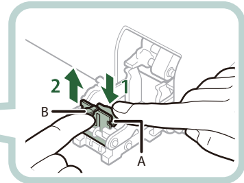
Saddle Stitcher Unit of the Booklet Finisher-P1 (p. 162)
