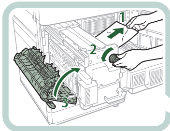
Fixing Transport Unit (p. 119)
