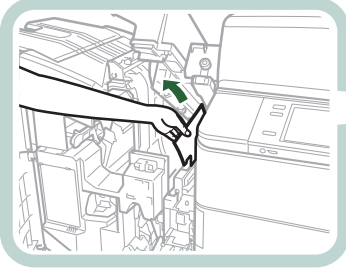
External 2 Hole Puncher-A1/External 2/3 Hole Puncher-A1/External 2/4 Hole Puncher-A1 (Optional) (p. 141)
