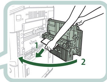
Multi-purpose Tray (p. 122)
