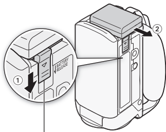
BATTERY RELEASE 开关
