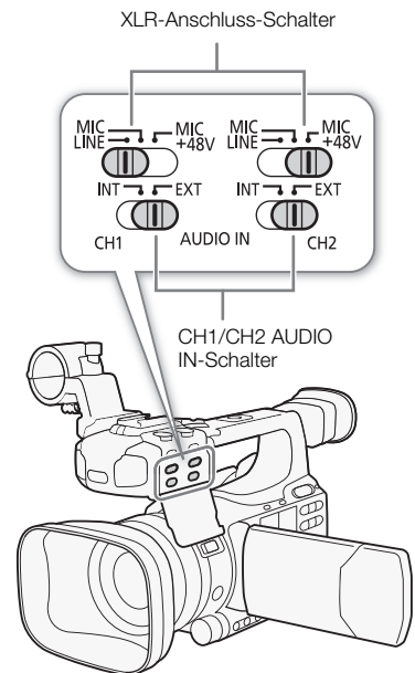
XLR-Anschlüsse
