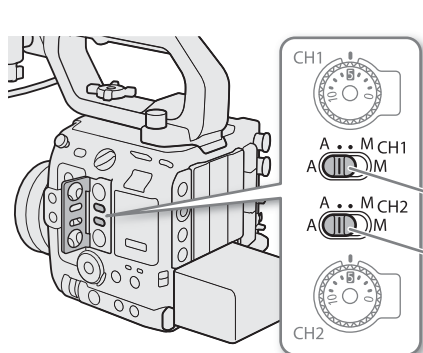
CH1/CH2 audio level switches
