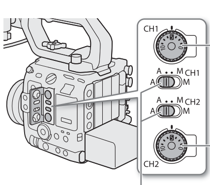
CH1/CH2 audio level dials
